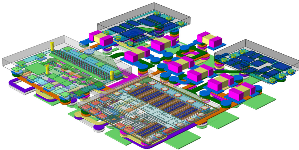
Figure 2: In module design, there are usually multiple technologies, as well as the PCB technology of the module itself
