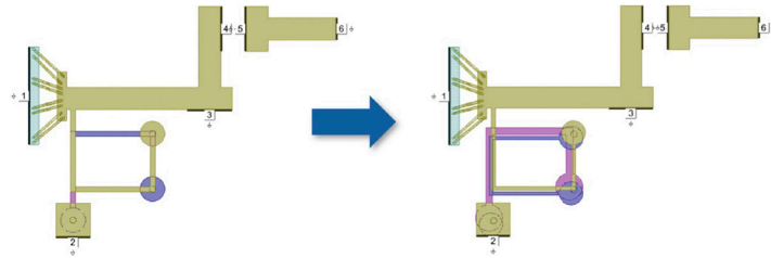
Figure 3: Metals are the same width/aligned on the Z-axis in the spiral inductor (left), and layers have shifted in X/Y independently of one another (right)
