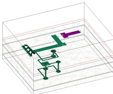
Figure 5: The connectivity highlighter in AWR Microwave Office software highlights if the metal connectivity is changing to ensure there are no opens or short in the circuit when using the layer modifiers tool
