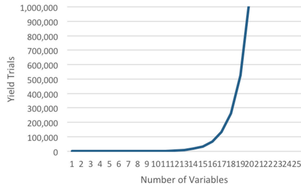
Figure 1: Required yield trials for corner analysis
