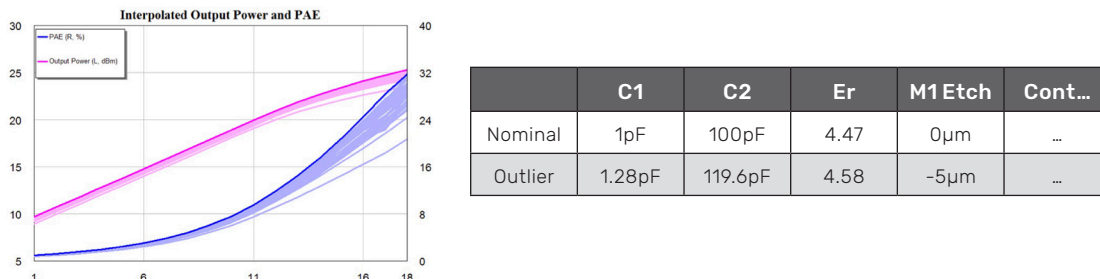
Figure 8: The actual PAE and output power for a yield analysis, where the impedances presented to the device were arbitrary and the output power and PAE were interpolated
