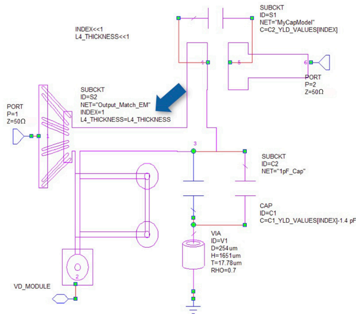
Figure 10: The PCB design can be exported to the Virtuoso environment, where the IC designer can optimize the PCB to the IC
