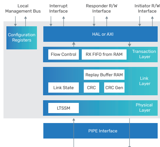
Figure 2: IP-level block diagram
