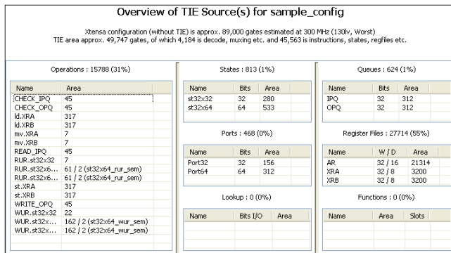
Figure 5: The TIE analyzer estimates gate count and silicon area for new instructions.
