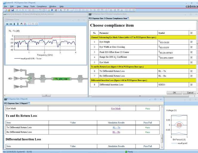
Figure 2: PCIe Gen3 SerDes simulation incorporating IBIS AMI models and accounting for back-channel simulations
