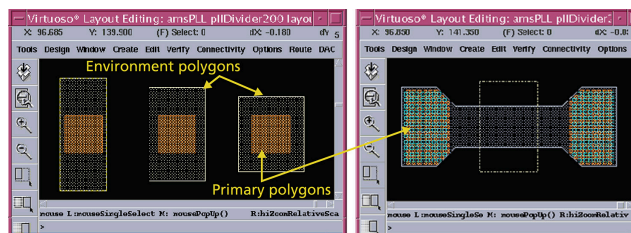
Figure 1: A set of design rules are described by drawings in a model file (GDSII, DFill, text vertices). A model contains a primary polygon (e.g., contact, fuse opening, DRC error markers) and environment polygons (e.g., metals enclosing contact, fuse metals/vias, waivable layout configuration per error marker). Pattern check is triggered by primary polygons in the design.
