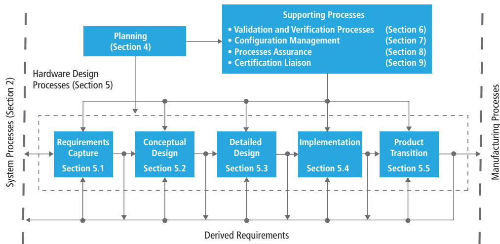
Figure 2: DO-254 flow
